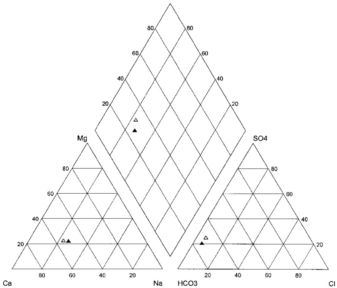
Figure 3. Davidson Samples June 4, 2002
