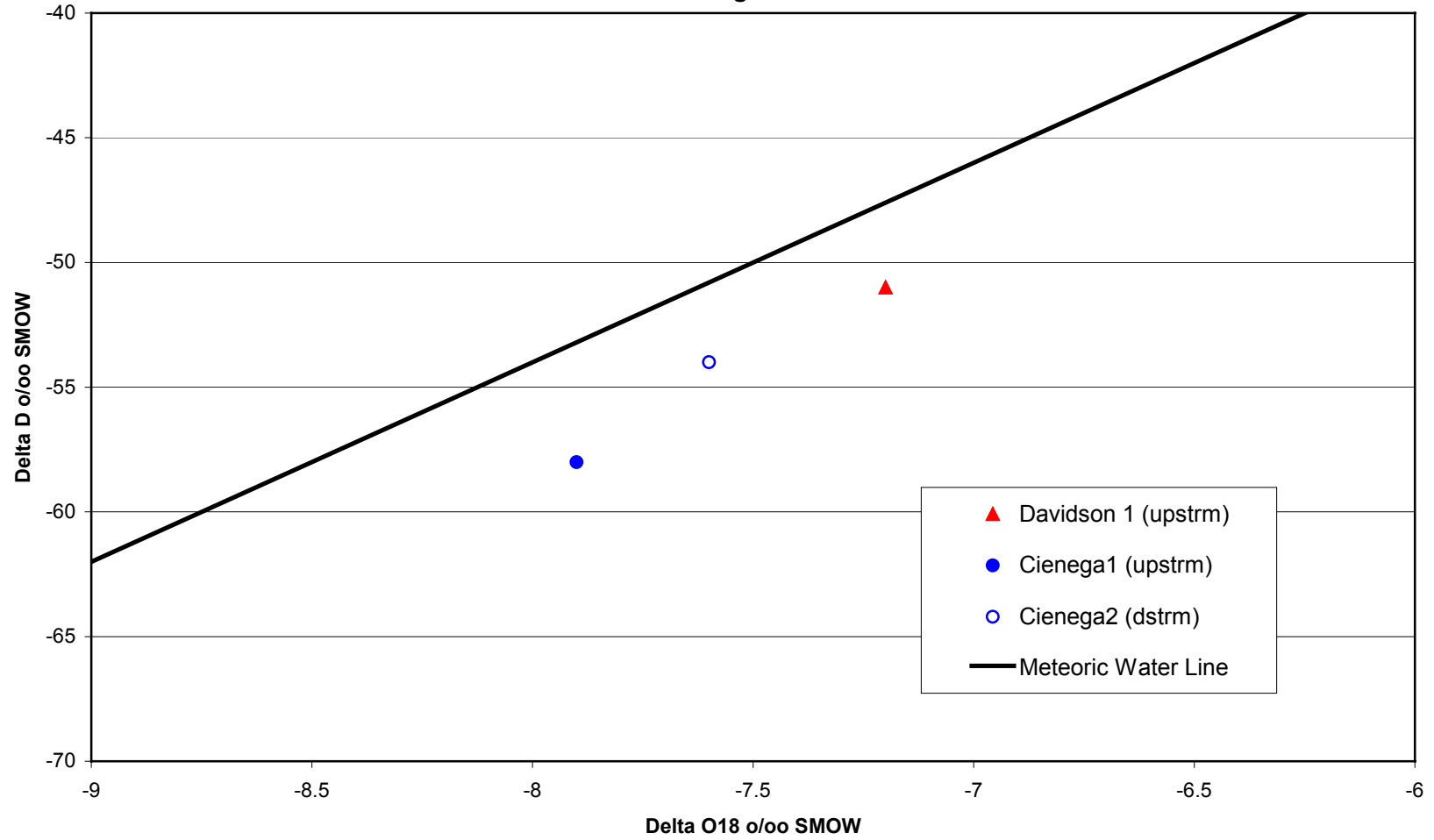
Figure 10. Cienega/Davidson Stable Isotope Sampling Results August 2002
