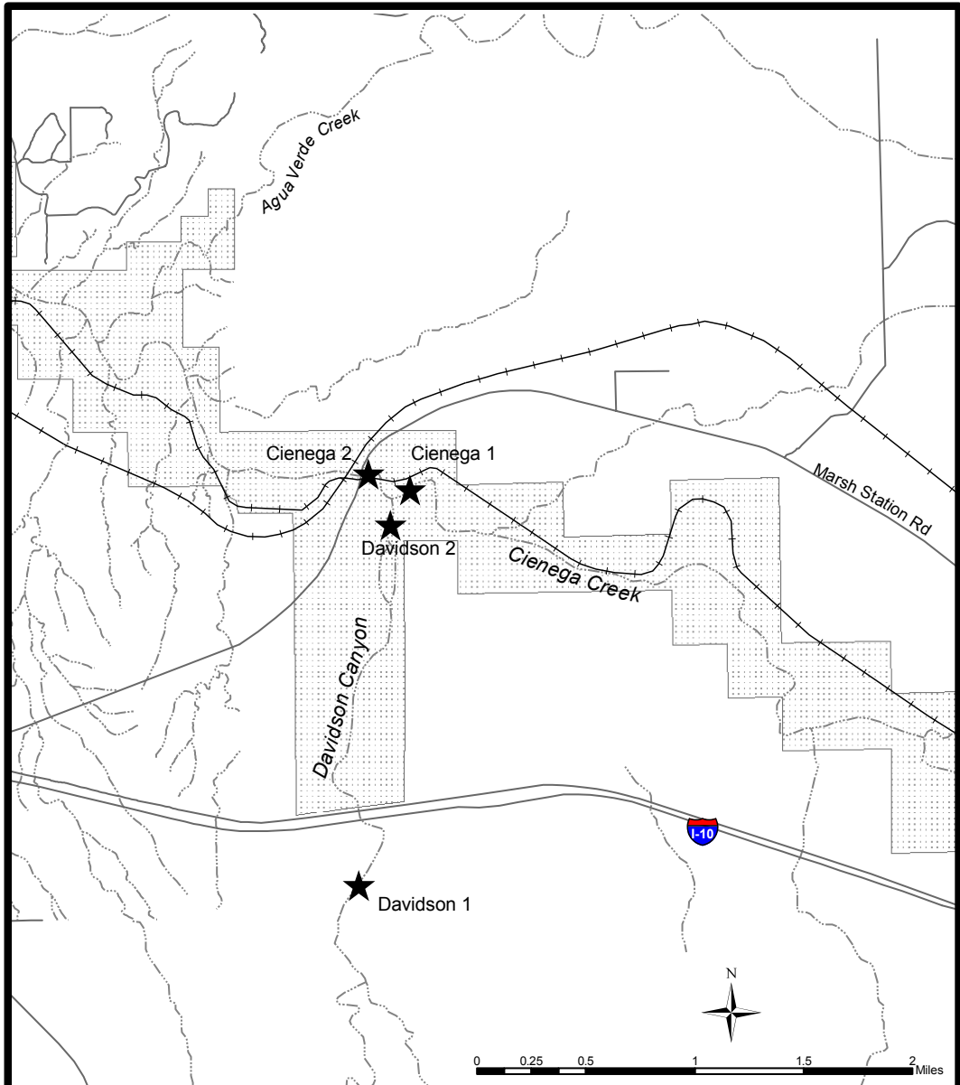
Figure 1. Sample Locations Along Davidson Canyon and Cienega Creek
