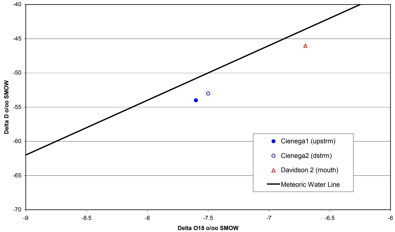
Figure 12. Cienega/Davidson Stable Isotope Sampling Results January 2003
