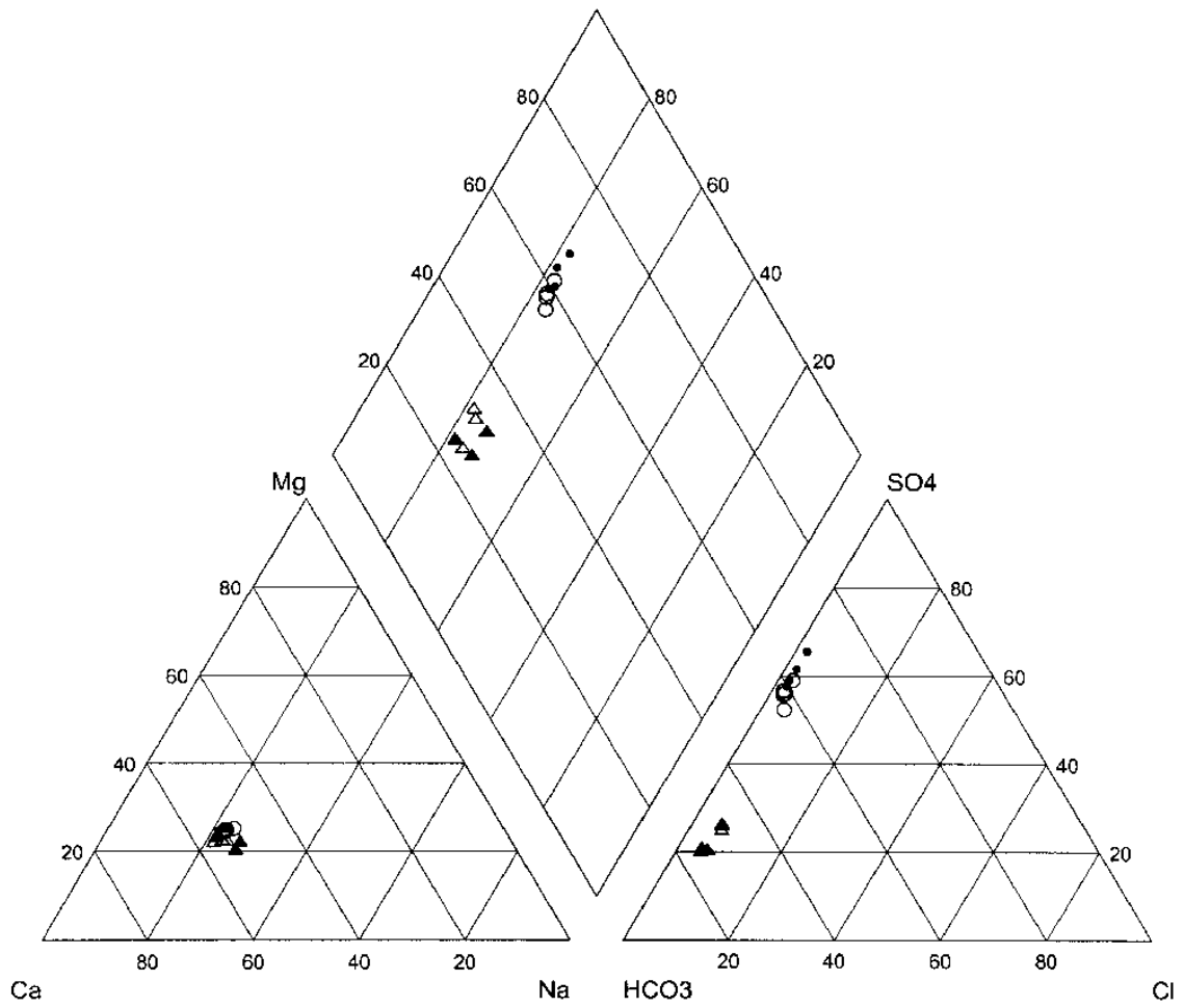
Figure 8. Piper Plot for All Samples
