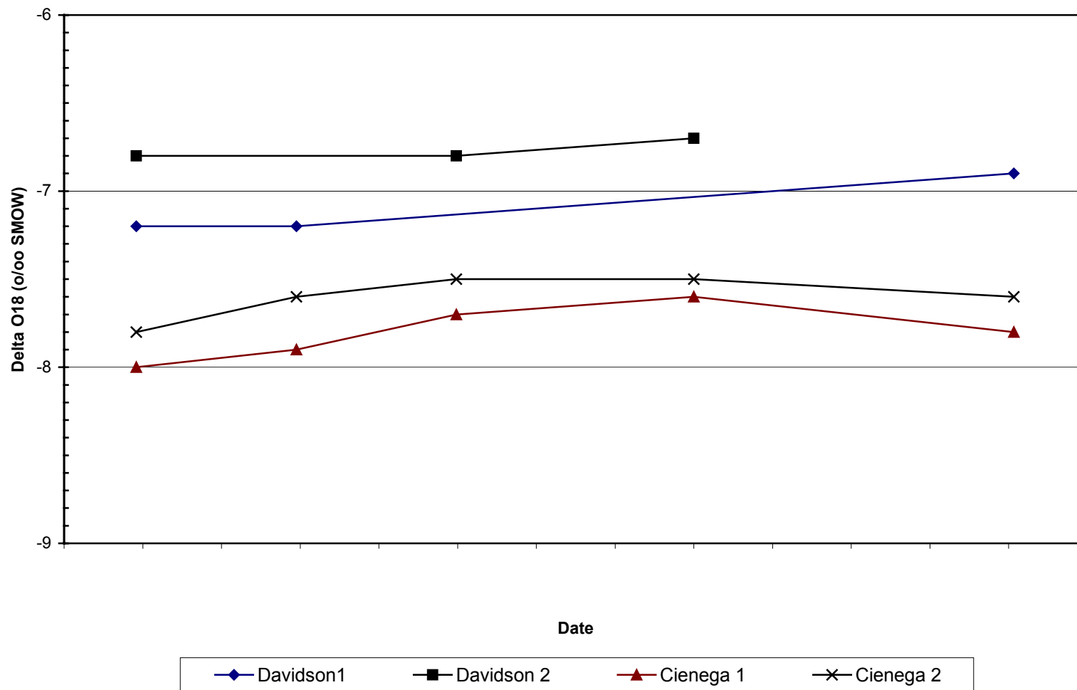
Figure 16. Cienega/Davidson Delta O18 Values
