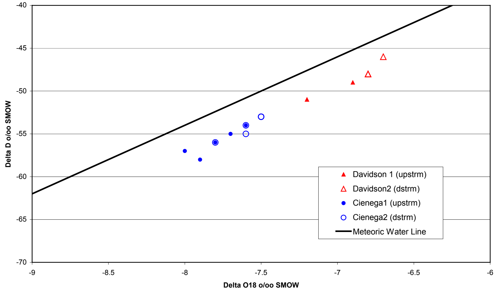
Figure 14. Cienega/Davidson Combined Stable Isotope Sampling Results
