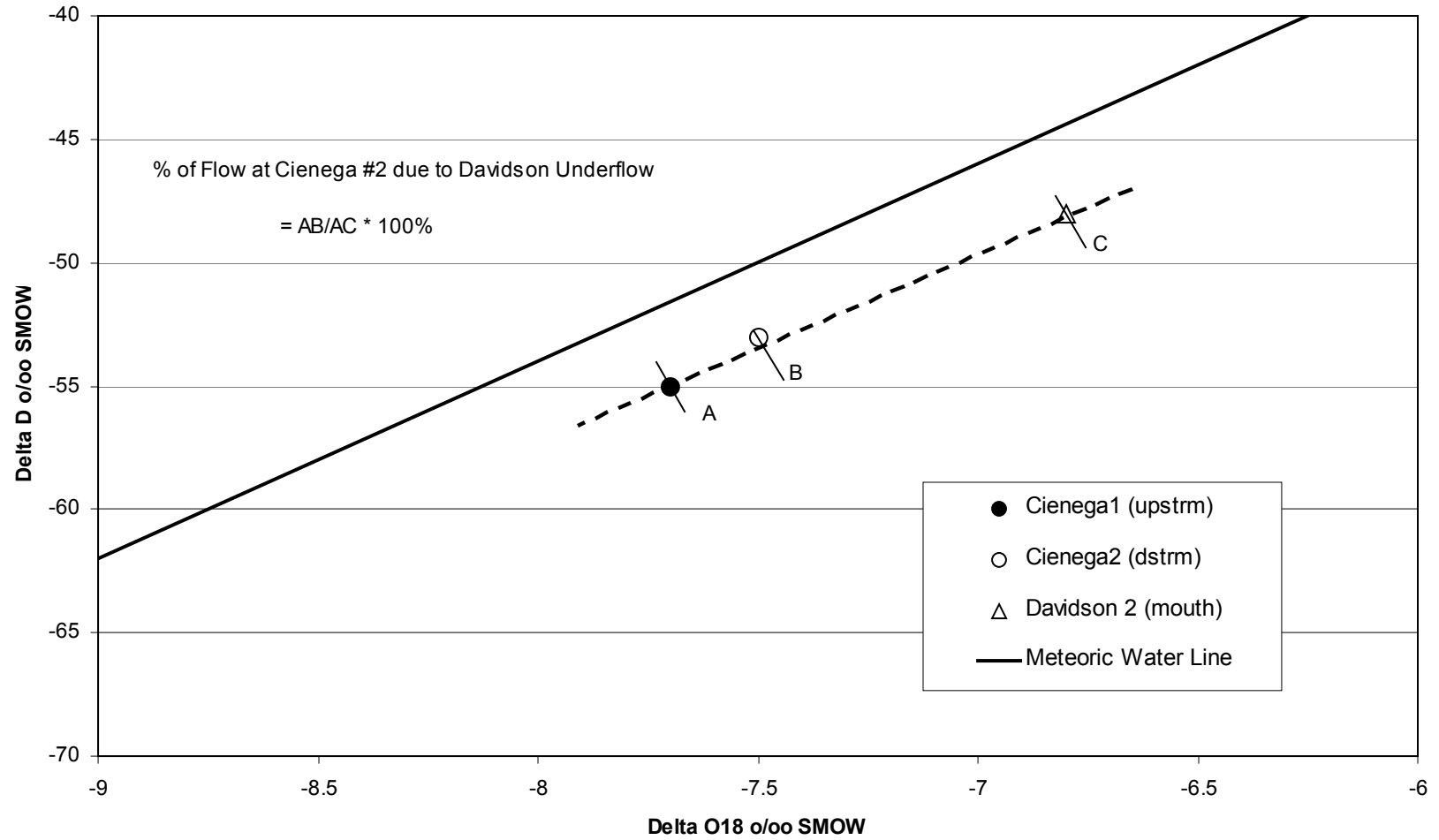
Figure 2. Calculation of Davidson Contribution from Stable Isotope Data
