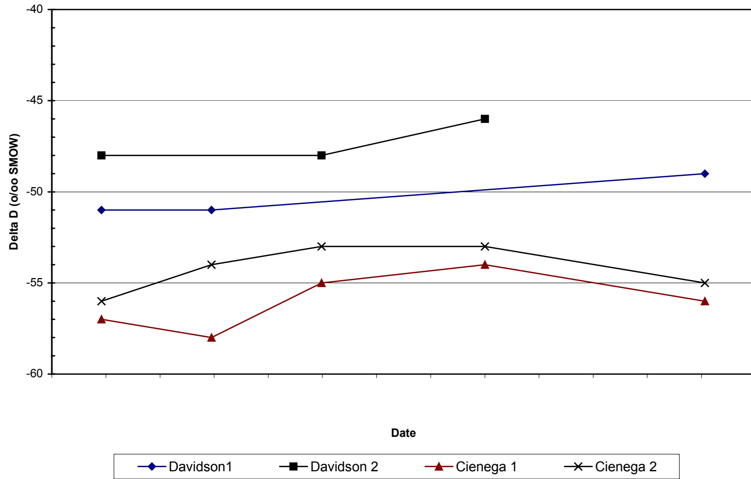
Figure 15. Cienega/Davidson Delta D Values
