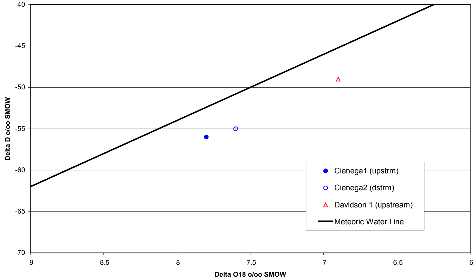
Figure 13. Cienega/Davidson Stable Isotope Sampling Results May 2003
